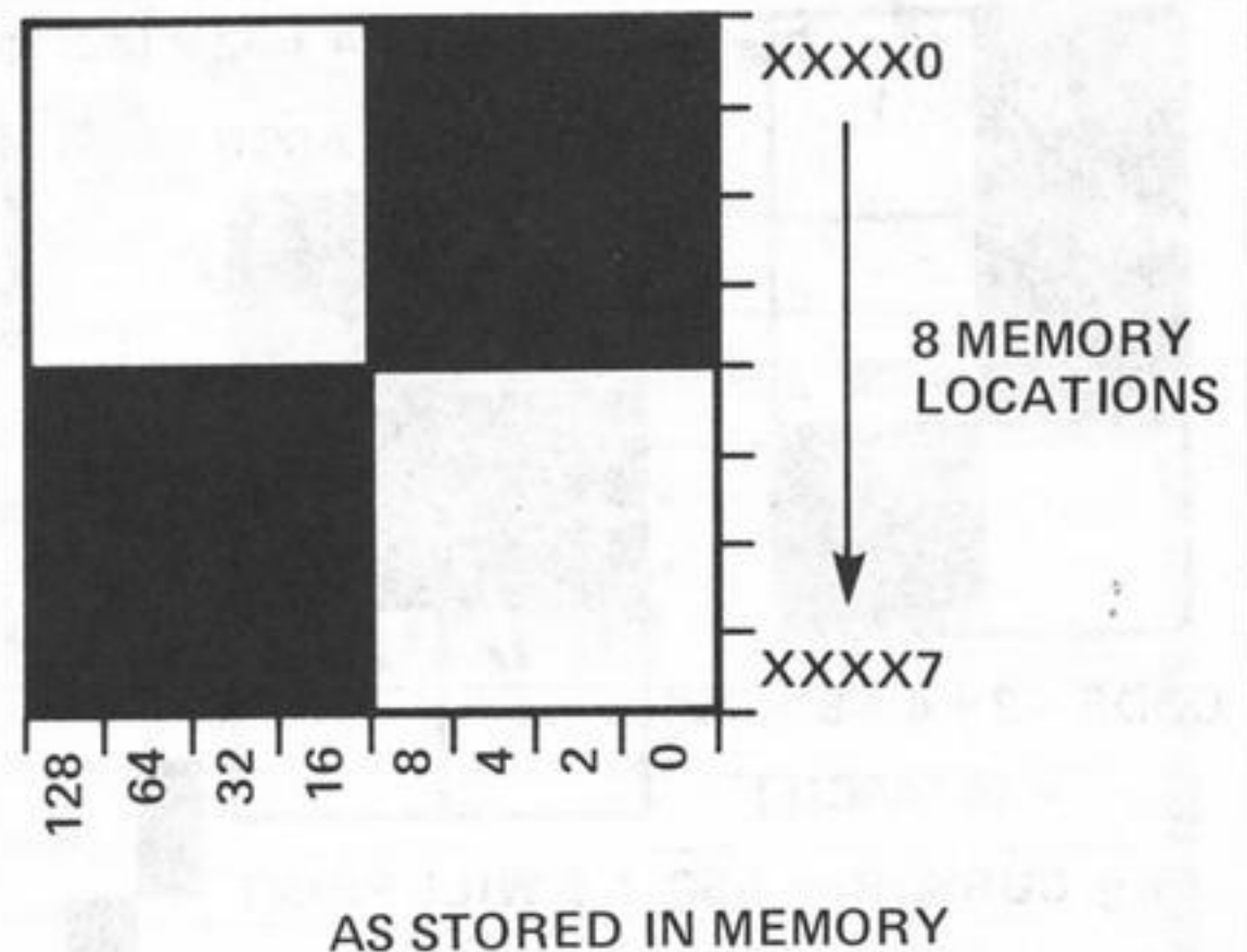
Figure 1 — how graphics are stored and displayed
